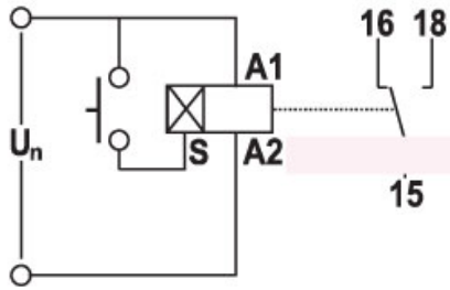
3-wire connection
